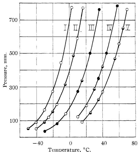
Fig. 1.—Vapor pressure: I, (CH 3 ) 2 SiF 2 ; II, (CH 3 ) 3 SiF; III, (CH 3 ) 2 SiClF; IV, (CH 3 ) 3 SiCl; V, (CH 3 ) 3 SiCl 2 . sample A, O; sample B, □; sample C, ●.
